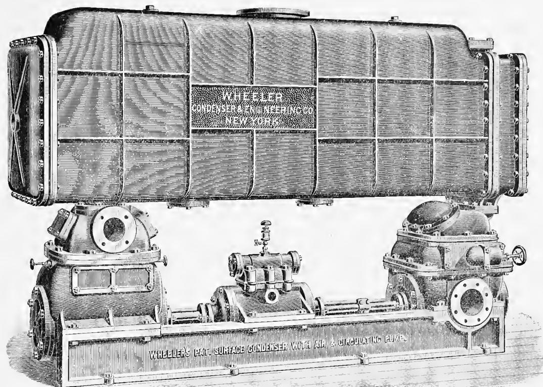
RECTANGULAR PATTERN OF THE WHEELER-ADMIRALTY SURFACE CONDENSER MOUNTED UPON COMBINED AIR AND CIRCULATING-PUMPS.
